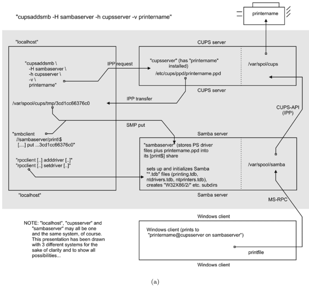
Figure 19.16. cupsaddsmb flowchart.
