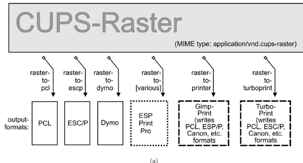
Figure 19.9. Raster to printer-specific formats.
