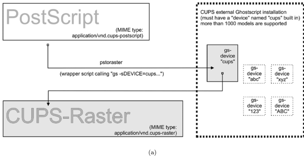
Figure 19.7. CUPS-raster production using Ghostscript.
